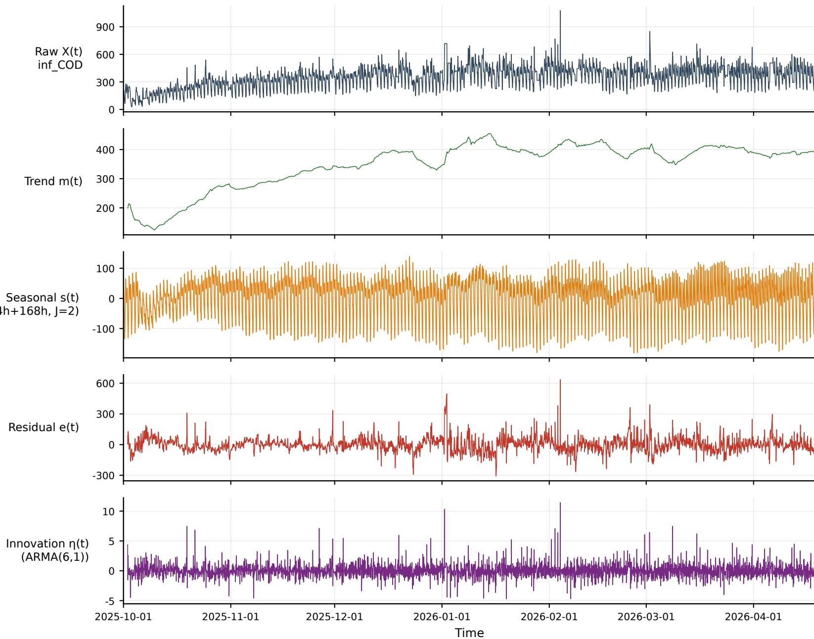
Multi-scale decomposition — inf_COD (influent, hour) [2025-10-01~2026-04-19]
